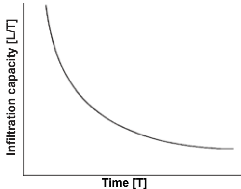
(Figure 4) - Infiltration Curve
