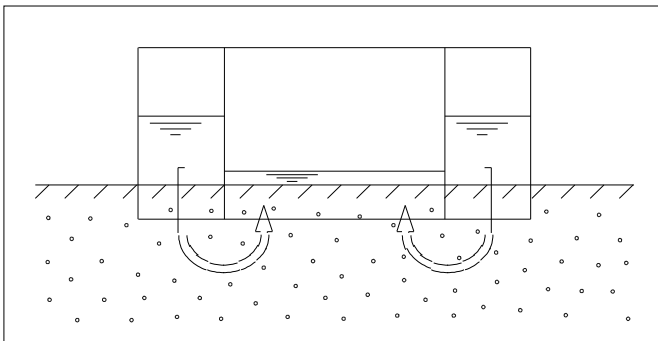
(Figure 6) Decreasing infiltration caused by different water levels in the inner and the outer rings.
